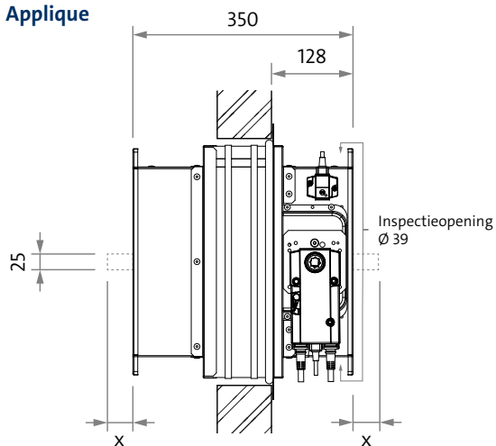
FD25 APP M
